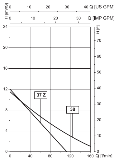
Motor F 414 in combination with pump tube sets in Aluminium or Hastelloy C
