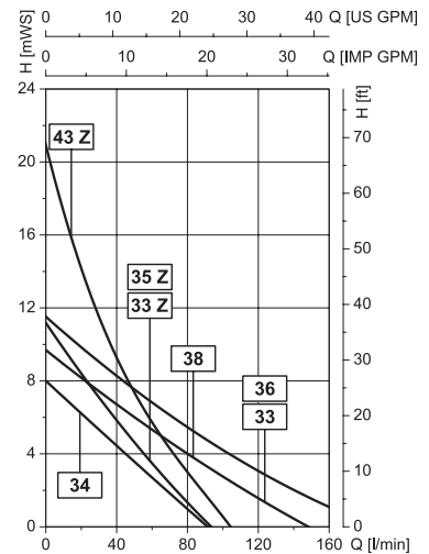
Motor F 414 in combination with pump tube sets in PP or PVDF
