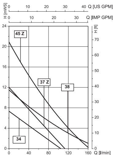
Motor F 414 in combination with pump tube sets in stainless steel
