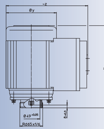
Single-phase motor (SPM) with capacitor switch, for use with F 550 GS6 and F 520 S-41/37
