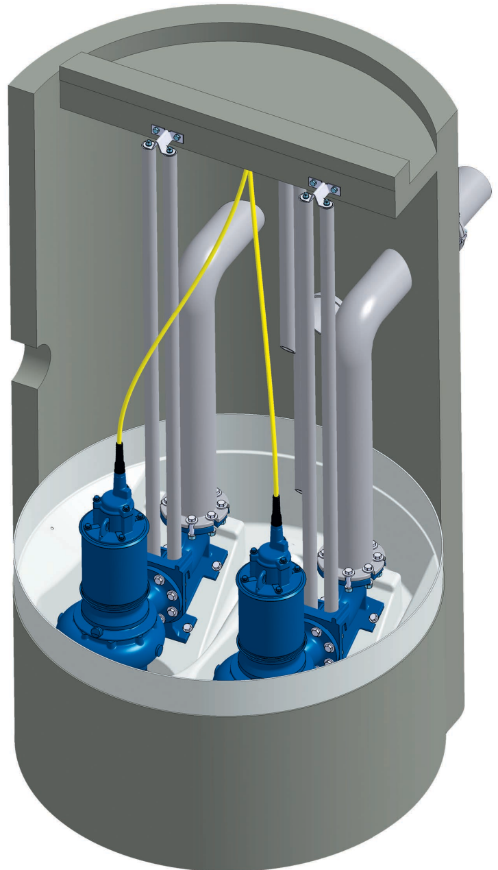
Section: Double basin pump sump
