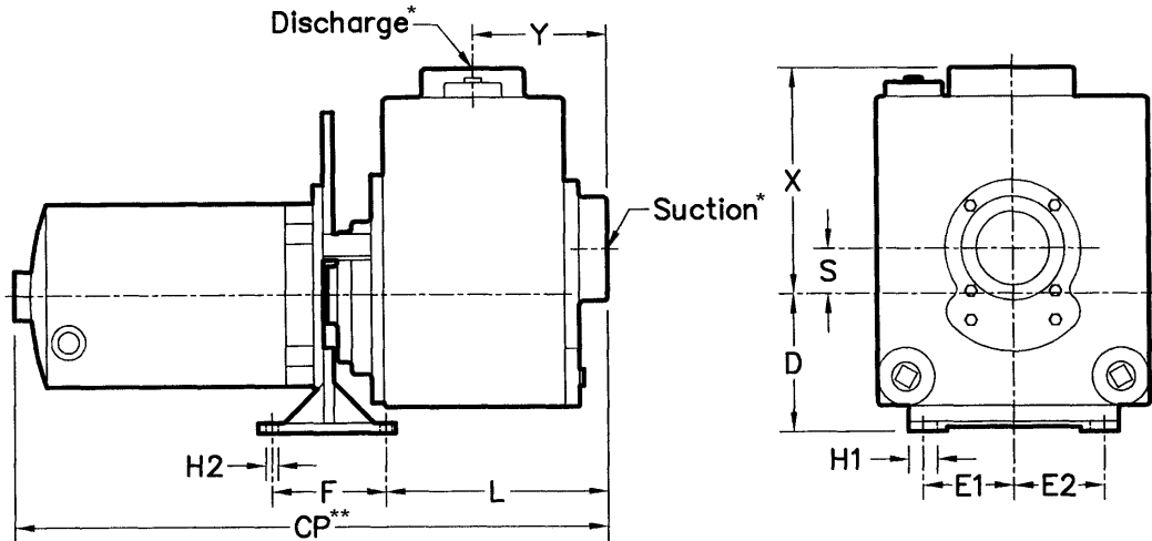
Pump Dimensional & Specification Chart
