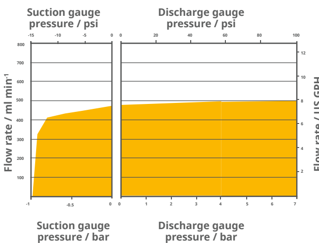
Flow rates based on pumping water at 20C with zero suction and delivery heads
